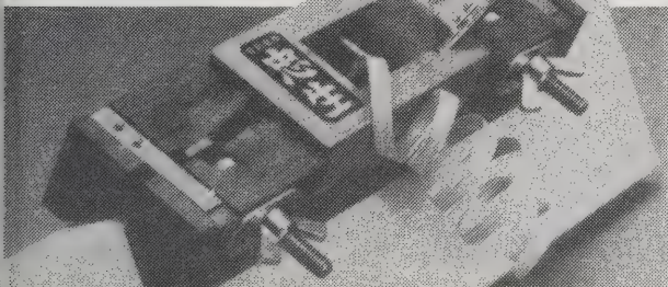
Adjustable chamfer plane (Mentori Ganna); Tadao brand.
